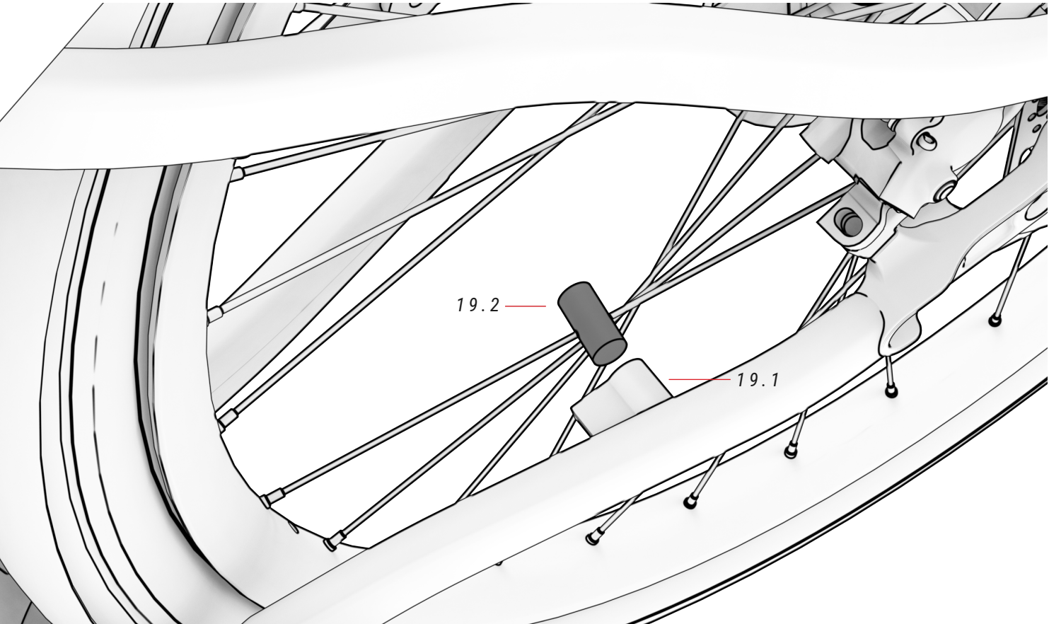
19 SPEED SENSOR MAGNET ref.:387332400
