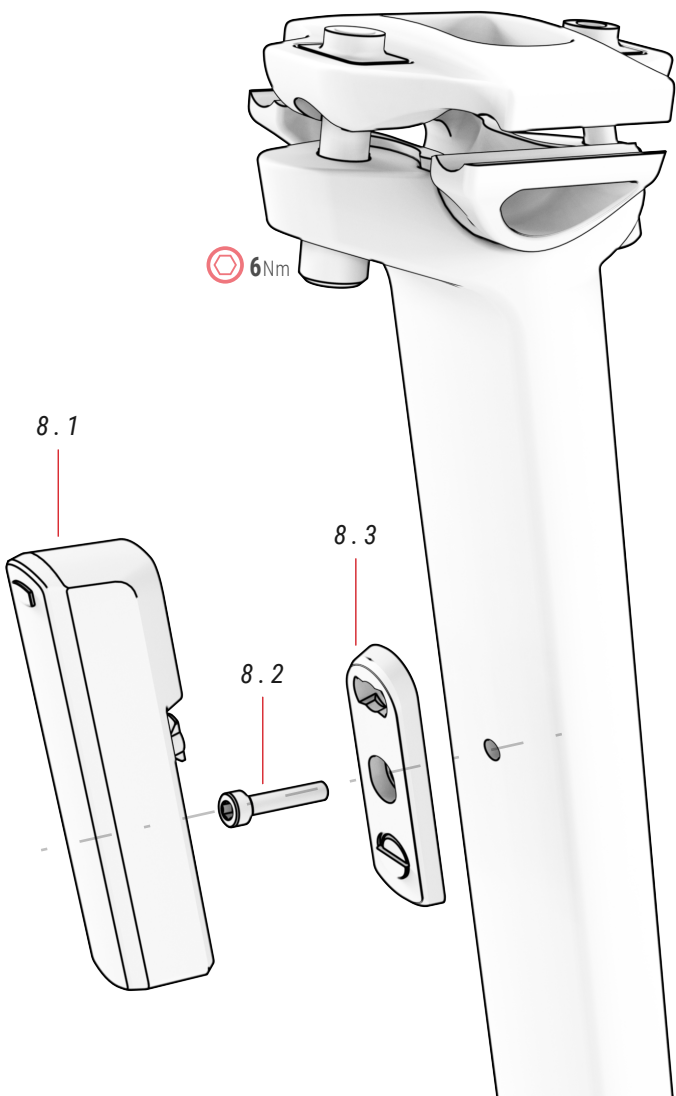
08 REAR LIGHT ref.: 387435700
