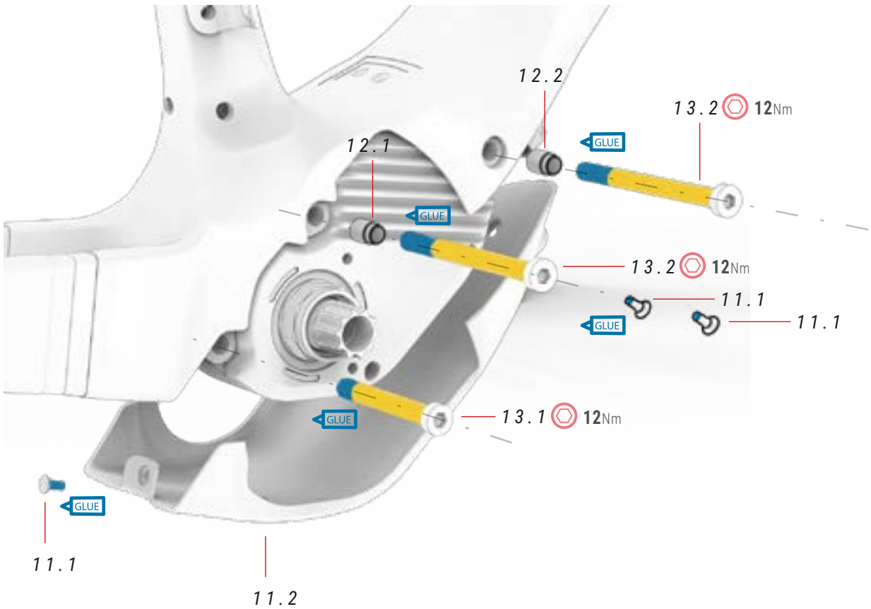
EC297 / EC287 / EC277 11 MOTOR COVER ref.: 391849400
