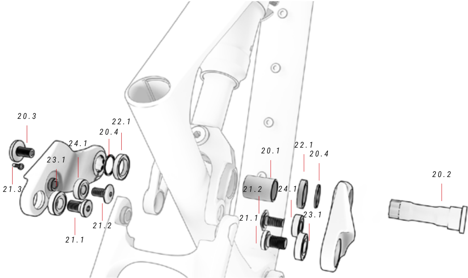
20 THRU AXLE BIELA ref.: 391834800
