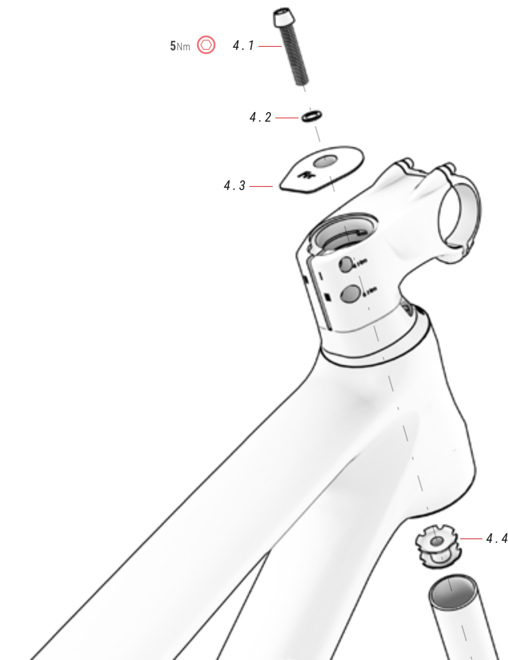
04 TAMPA ref.: 363297300
